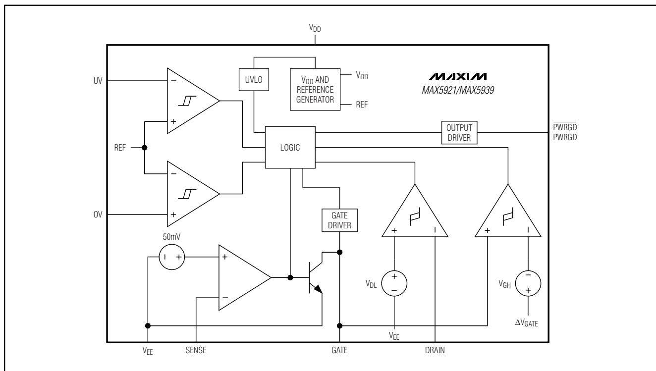
Block Diagram
