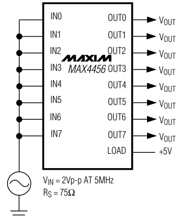
ALL-CHANNEL OFF-ISOLATION (NOTES 1, 5–8)
