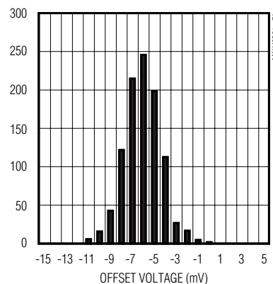
OFFSET VOLTAGE DISTRIBUTION
