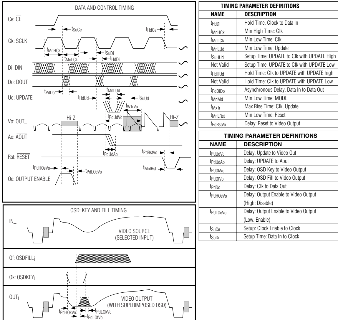
Figure 1. Timing Diagram
