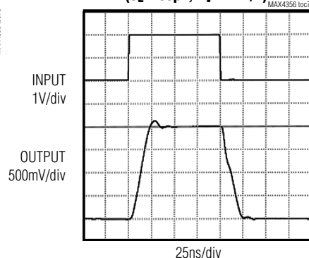
LARGE-SIGNAL PULSE RESPONSE WITH CAPACITIVE LOAD ( C_L = 30pF , A_V = +1V/V )
