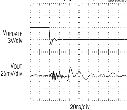
SWITCHING TRANSIENT (GLITCH) ( A_V = +2V/V )
