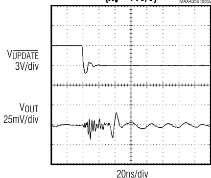
SWITCHING TRANSIENT (GLITCH) ( A_V = +1V/V )
