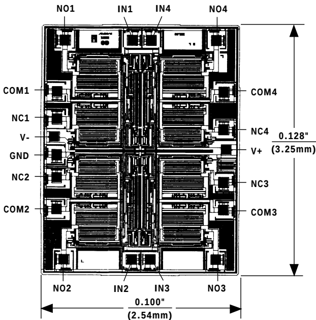
Chip Topography
