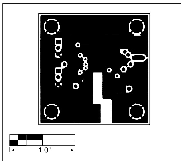
Figure 6. MAX2264/MAX2265 EV Kits PC Board Layout—Ground Plane
