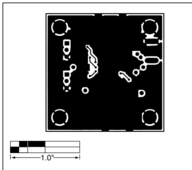
Figure 8. MAX2264/MAX2265 EV Kits PC Board Layout—Solder Side
