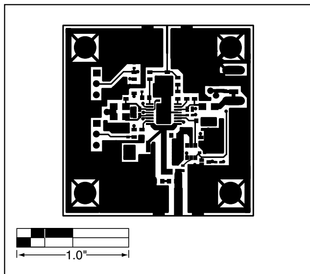
Figure 10. MAX2266 EV Kit PC Board Layout—Component Side
