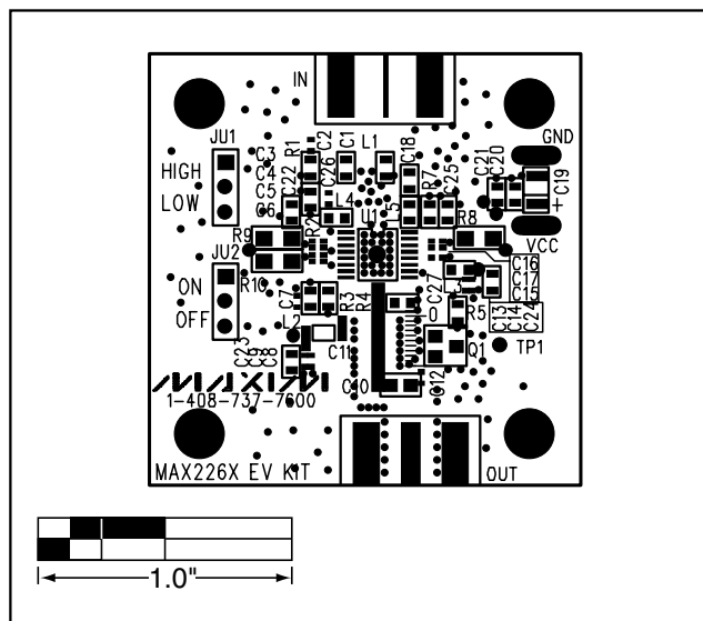
Figure 4. MAX2264/MAX2265 EV Kits—Component Placement Guide
