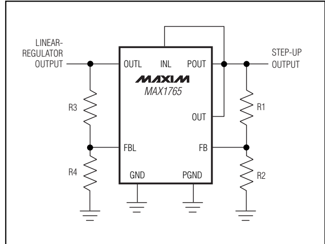
Figure 7. Feedback Connections
