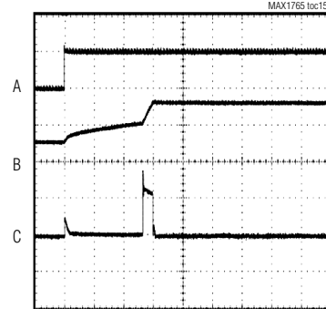
TURN-ON WAVEFORMS NO SOFT-START COMPONENTS
