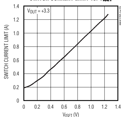
SWITCH CURRENT LIMIT vs. V_{ISET}
