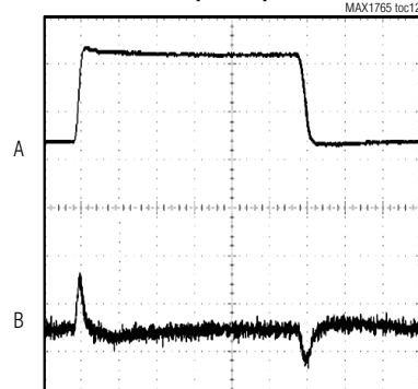
LINE TRANSIENT RESPONSE (DC-DC)
