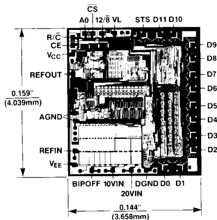
Chip Topography
