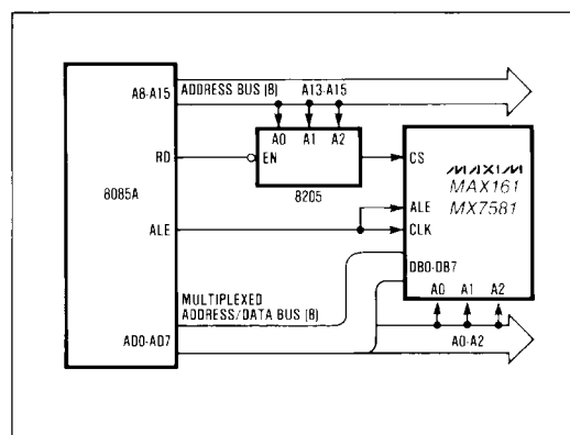
Figure 11. 8085A Interface
