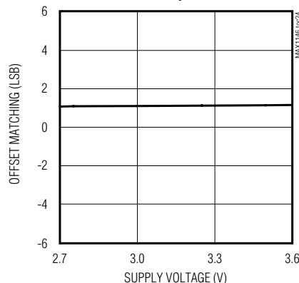
CHANNEL-TO-CHANNEL OFFSET MATCHING vs. SUPPLY VOLTAGE (MAX1147/MAX1149)
