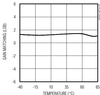
CHANNEL-TO-CHANNEL GAIN MATCHING vs. TEMPERATURE
