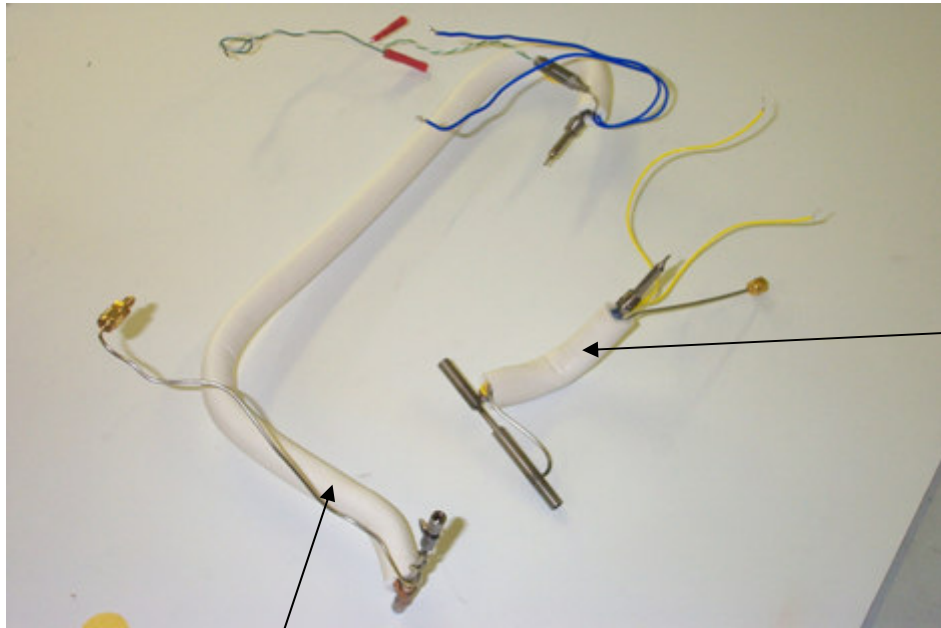
Recollection Heated Link MTD-1227
