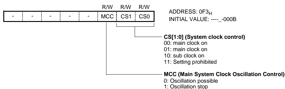
SCMR (System Clock Mode Register)
