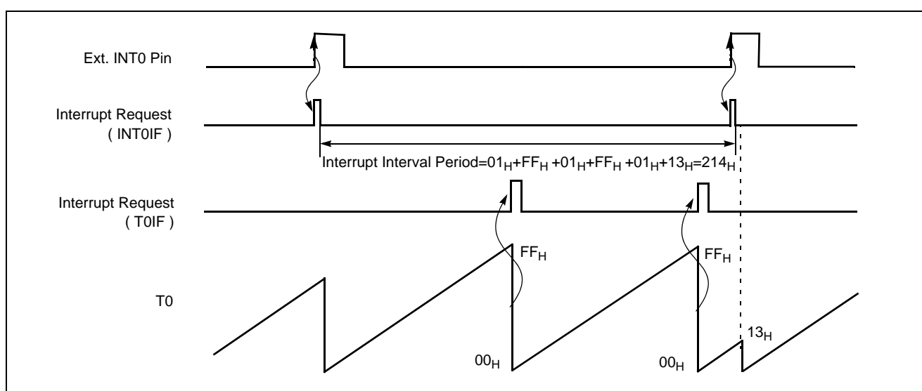
Figure 14-16 Excess Timer Overflow in Capture Mode
