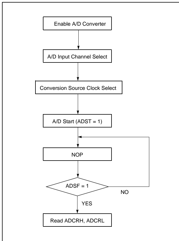
Figure 15-1 A/D Converter Operation Flow
