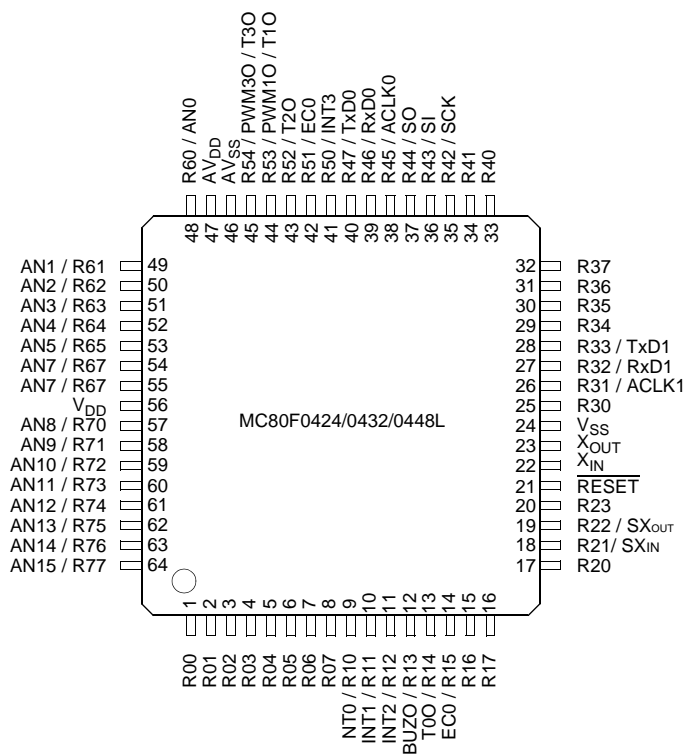
64LQFP (Top View)
