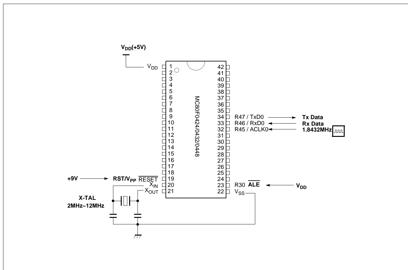
Figure 27-1 ISP Configuration
