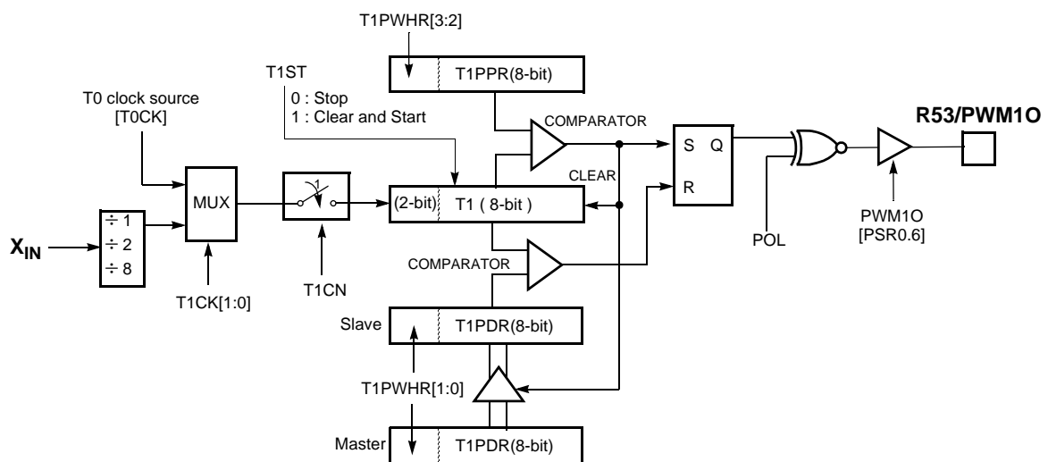
Figure 14-20 PWM1 Mode
