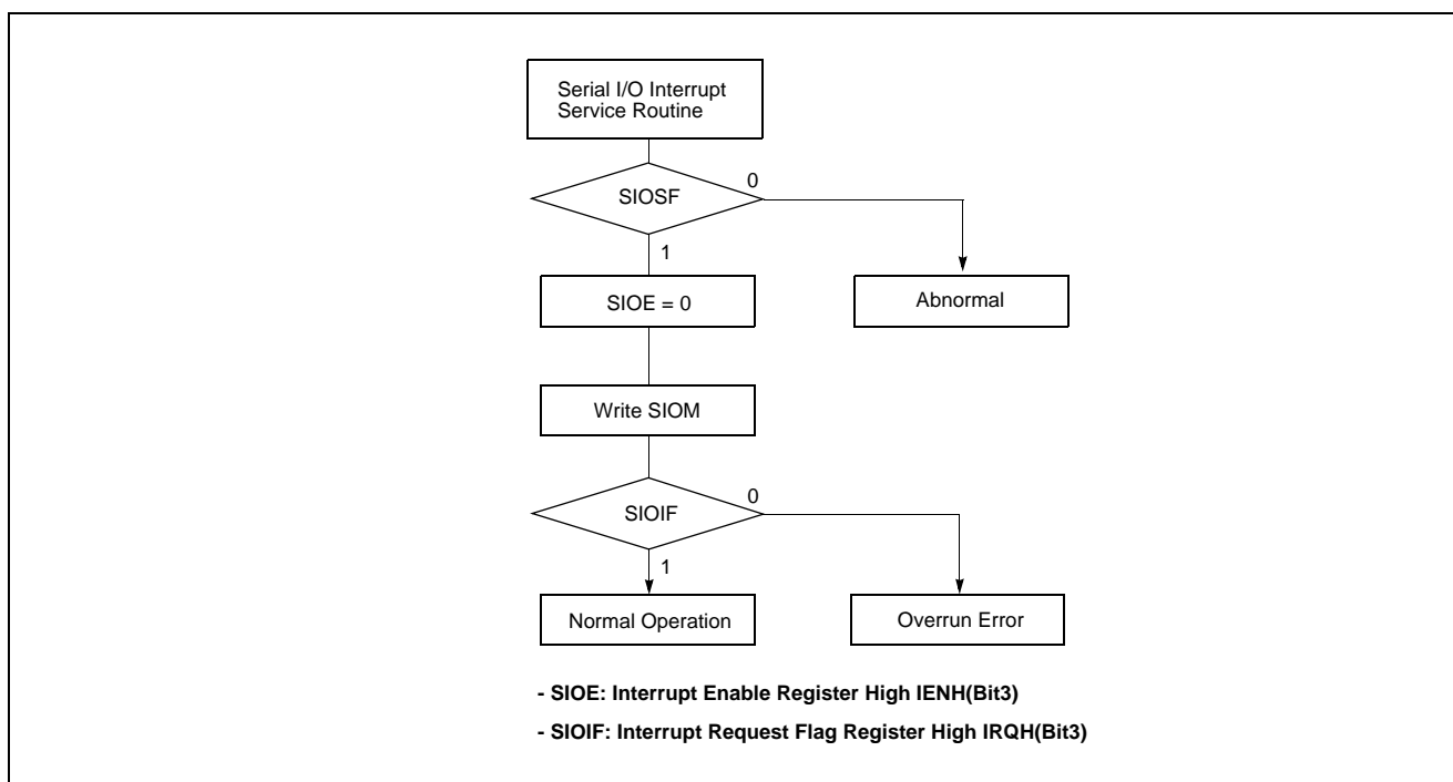
Figure 16-5 Serial IO Method to Test Transmission
