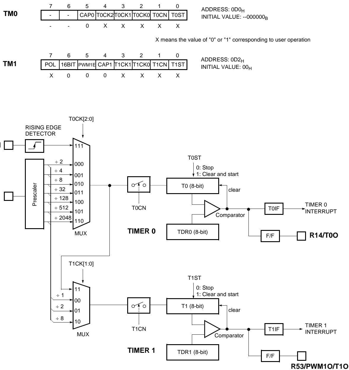
Figure 14-4 8-bit Timer/Counter 0, 1
