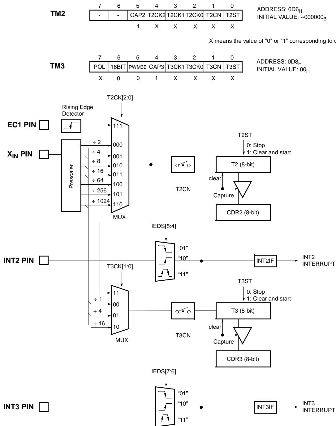
Figure 14-14 8-bit Capture Mode for Timer 2, 3
