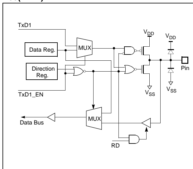
R33(TxD1)
