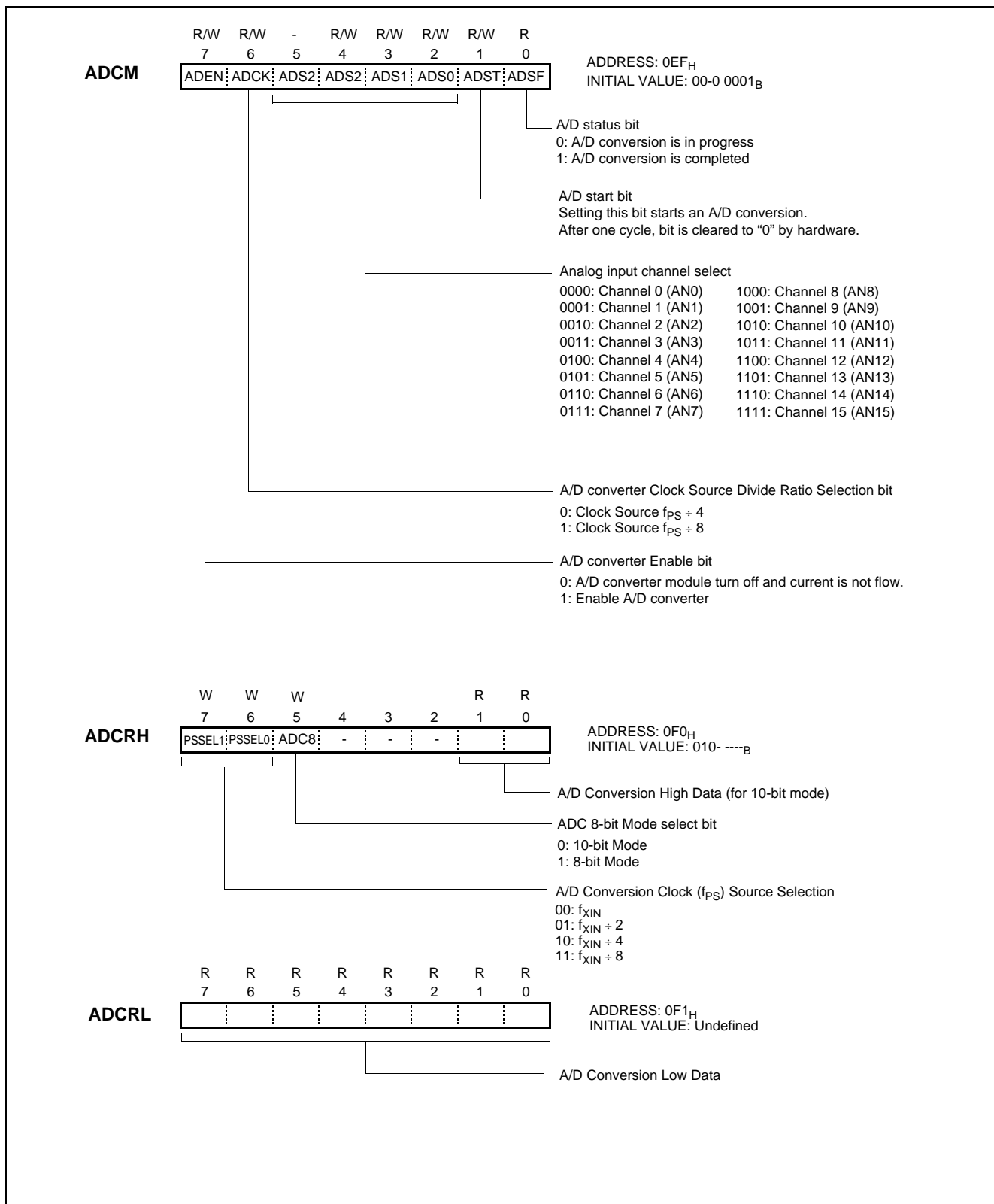
Figure 15-4 A/D Converter Control &amp; Result Register
