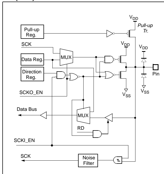
R42(SCK)
