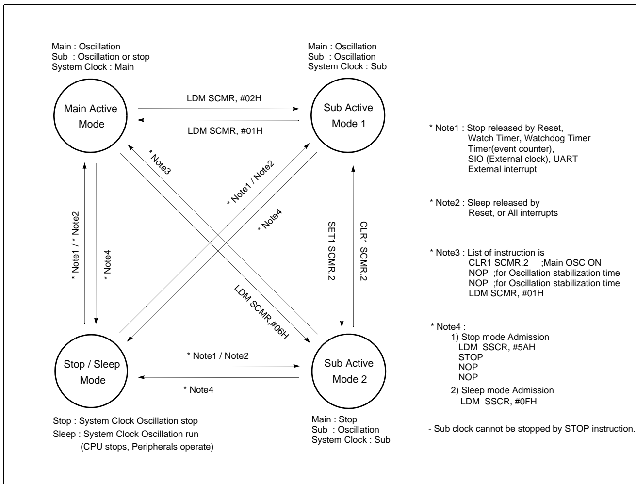
Figure 20-1 Operating Mode
