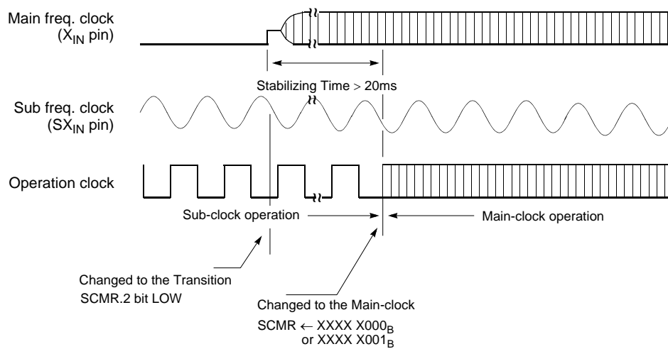
(b) Sub active mode 2 \rightarrow Sub active mode 1 \rightarrow Main active mode
