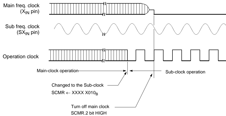
(a) Main active mode \rightarrow Sub active mode 1 \rightarrow Sub active mode 2
