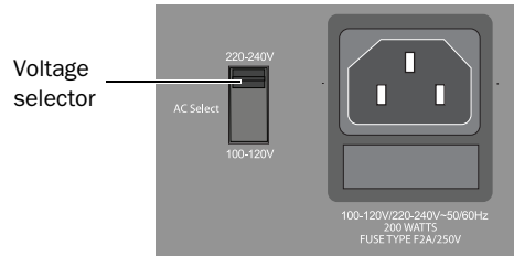
Voltage selector
