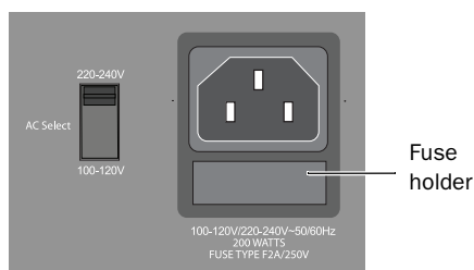
Fuse holder
