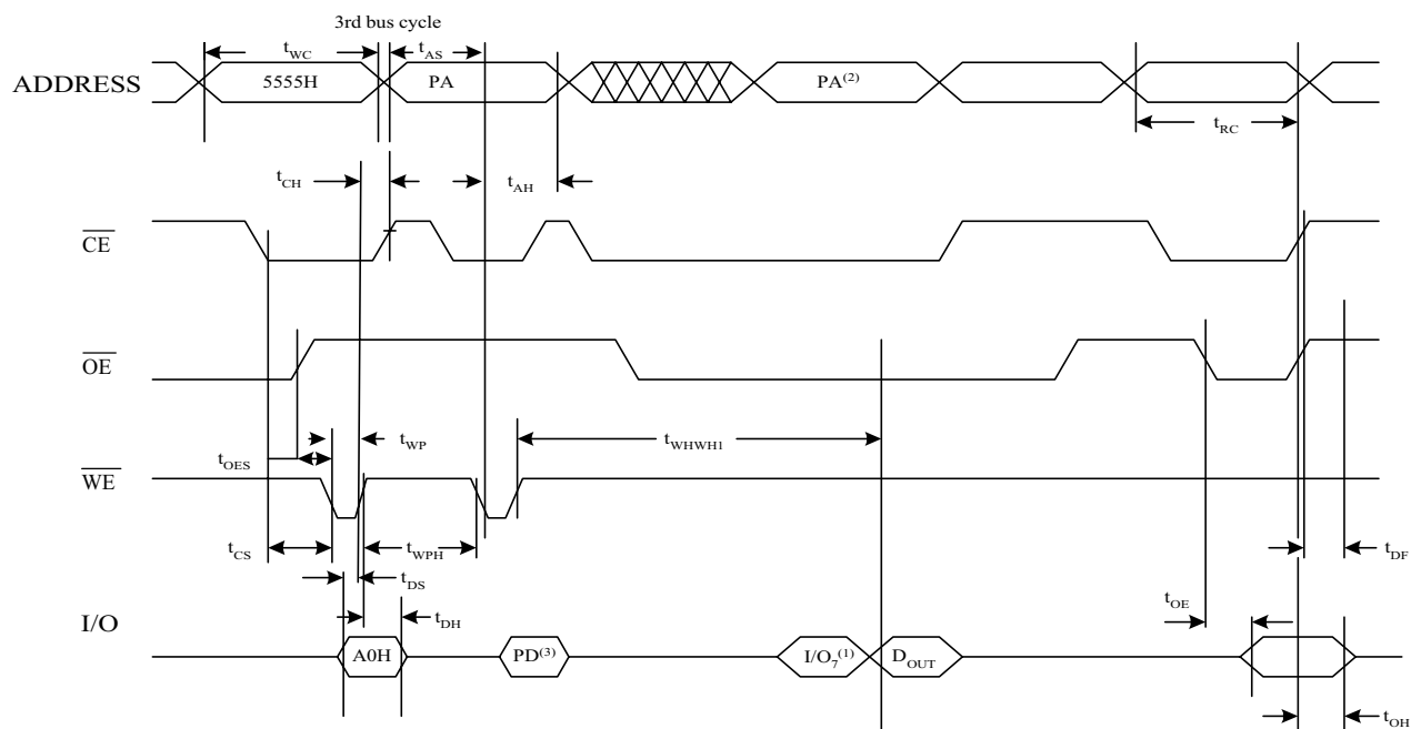
Waveforms of \overline{WE} Controlled-Program Cycle
