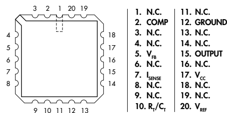
L PACKAGE (Top View)
