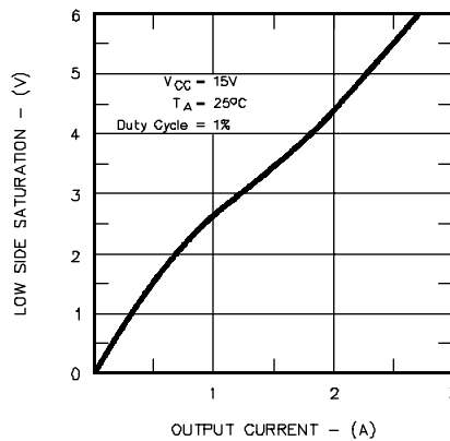
FIGURE 9. LOW SIDE SATURATION VS. OUTPUT CURRENT
