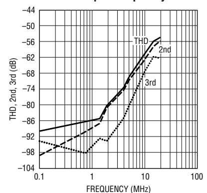
THD, 2nd and 3rd vs Input Frequency
