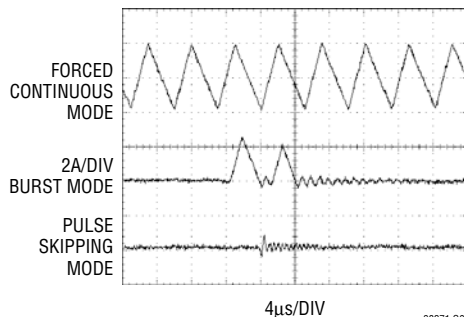
FIGURE 13 CIRCUIT V OUT = 3.3V I LOAD = 300μA
