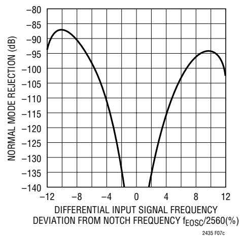
Figure 7c. LTC2435/LTC2435-1 Normal Mode Rejection When Using an External Oscillator of Frequency f_{\text{EOSC}} with Running Averages
