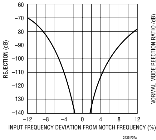
Figure 7a. LTC2435/LTC2435-1 Normal Mode Rejection When Using an External Oscillator of Frequency f_{\text{EOSC}} without Running Averages
