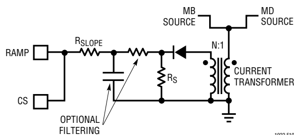
Figure 10. Current Transformer Sense Circuitry
