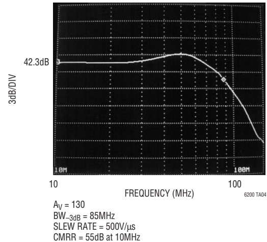
Instrumentation Amplifier Frequency Response
