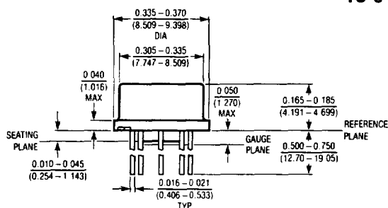
H Package TO-5 Metal Can
