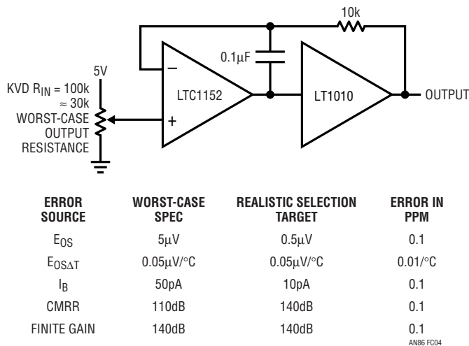
Figure C4. Error Budget Analysis for the KVD Buffer. Selection Permits ≈0.4ppm Predicted Linearity Error
