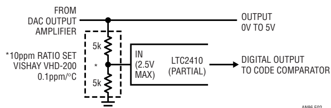
Figure E2. Precision Resistor Ratio Set Divides DAC Output, Permitting Higher Inherent Linearity LTC2410 Utilization. Disadvantage Is 5ppm/Yr and 0.1\text{ppm}/^\circ\text{C} Additional Drift Terms
