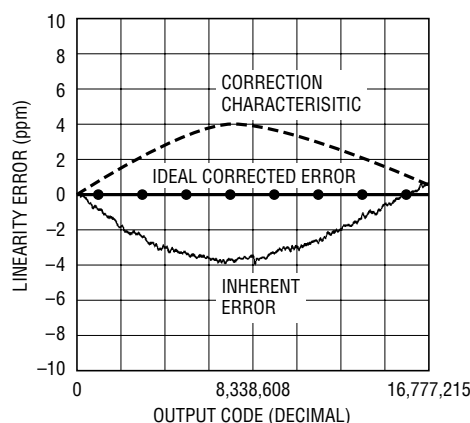
Figure E1. LTC2400 A-to-D Inherent Residual Linearity Error (Lower), Correction Characteristic (Upper) and Resultant Corrected Linearity (Center). Correction Ensures <1ppm Nonlinearity
