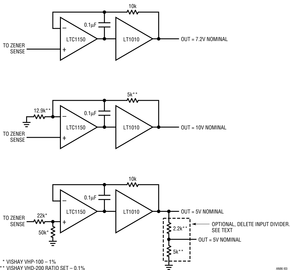
Figure I3. Chopper Stabilized Reference Buffer Options Include Unity Gain (a), 10V (b) and 5V (c) Output. Trimming Is Required for Absolute Accuracy
