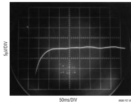
Figure 7. Small Step Settling Time Measures 100 Milliseconds to Within 1ppm ( \pm 5\mu\text{V} ) for a 500µV Transition
