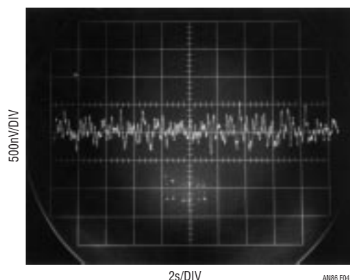
Figure H2. Indicated DAC Output Noise in a 0.1Hz to 10Hz Bandpass Is Below 1 \mu V, About 0.2LSB. Equipment Limitations Set Measurement Noise Floor at 0.2 \mu V
