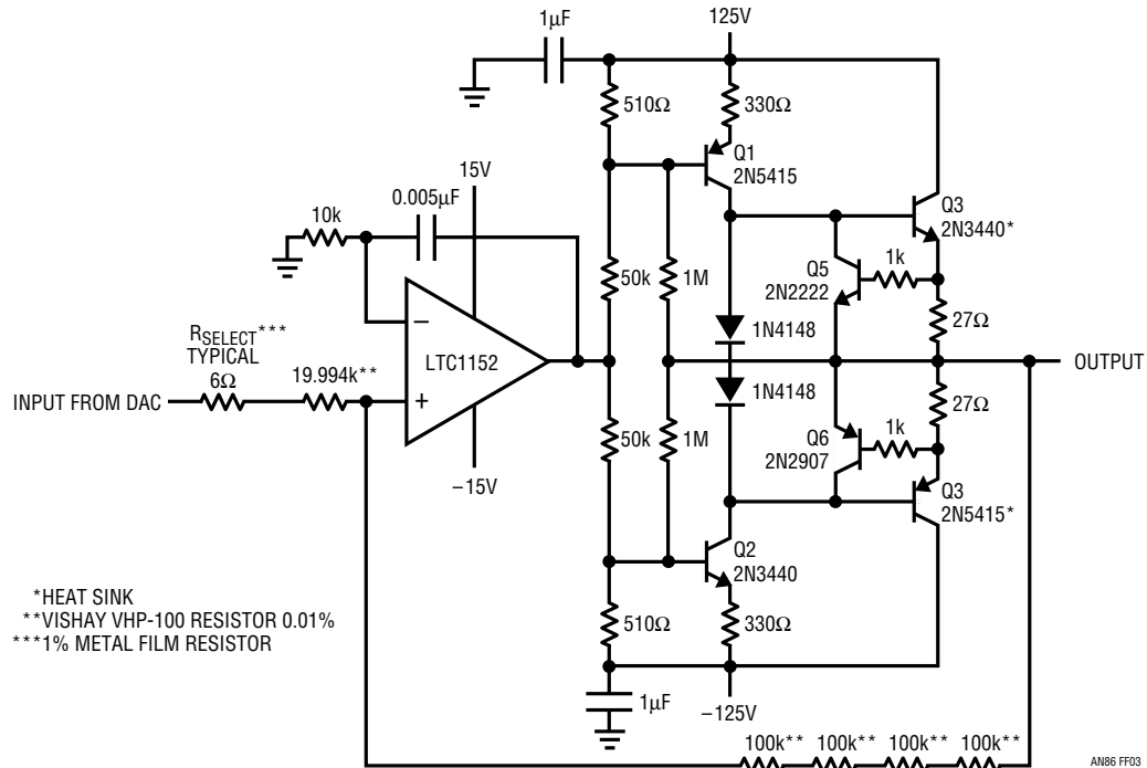
Figure F3. High Voltage Output Stage Delivers \pm 100\text{V} at 25\text{mA} . Multiple Feedback Resistors Minimize Dissipation and Voltage Coefficient Effects
