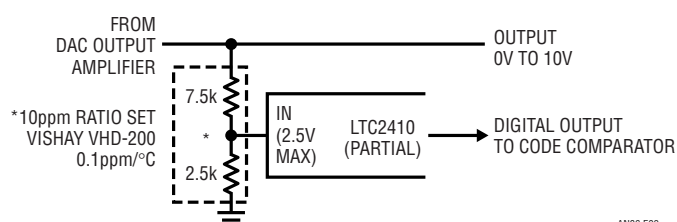
Figure E3. Similar to Figure E2, Except 3:1 Ratio Set Permits 10V Output While Accommodating LTC2410's 2.5V Input
