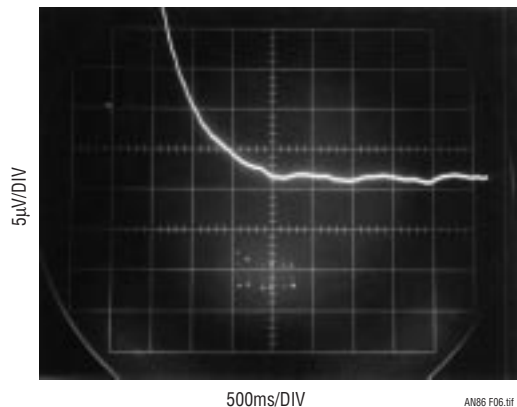
Figure 6. High Resolution Settling Detail After a Full-Scale Step. Settling Time Is 1400 Milliseconds to Within 1ppm ( \pm 5\mu\text{V} )
