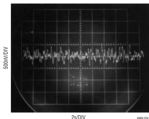
Figure 4. Output Noise Indicates Less Than 1 \mu V, About 0.2LSB. Measurement Noise Floor, Due to Equipment Limitations, Is 0.2 \mu V
