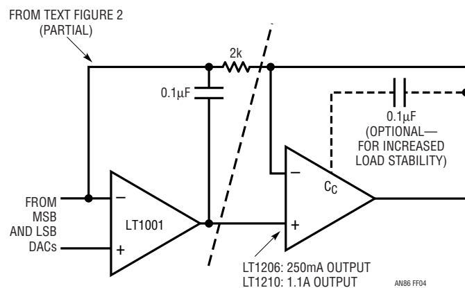
Figure F4. LT1206/LT1210 Output Stages Supply 250\text{mA} and 1.1\text{A} Loads, Respectively. Remote Sensing Is Usually Necessary to Compensate IR Drops
