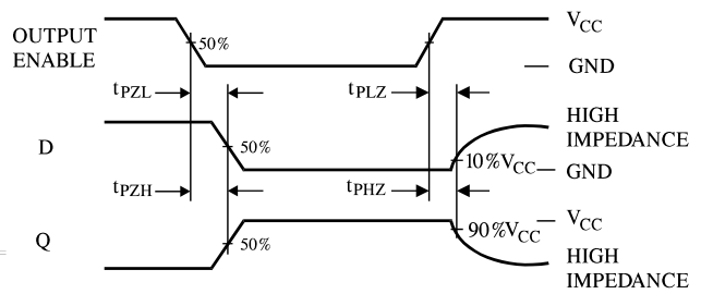
Figure 2. Switching Waveforms
