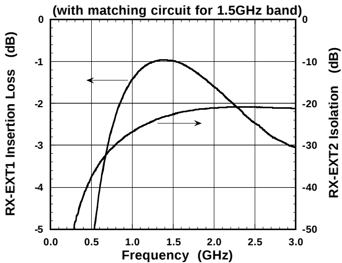
RX-EXT1 Insertion Loss RX-EXT2 Isolation (with matching circuit for 1.5GHz band)
