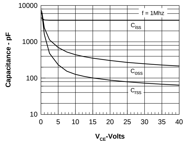
Figure 6. Capacitance Curves
