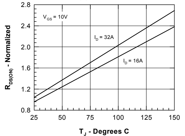
Figure 4. R_{DS(on)} normalized to 15A/25°C vs. T_J
