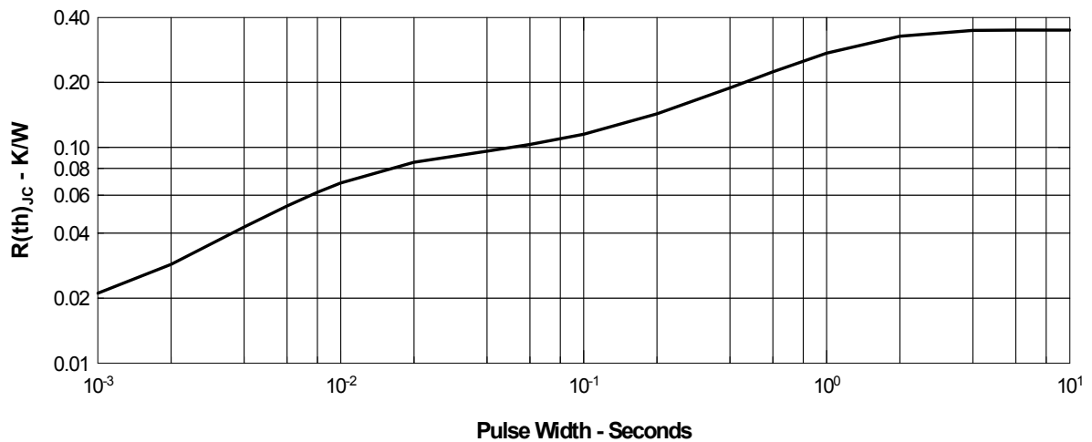
Figure 10. Transient Thermal Resistance
