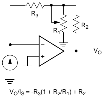
I to V Converter
