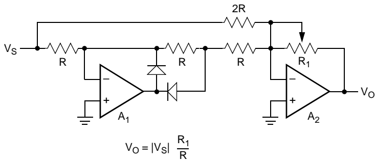
Absolute Value Amplifier with Gain
