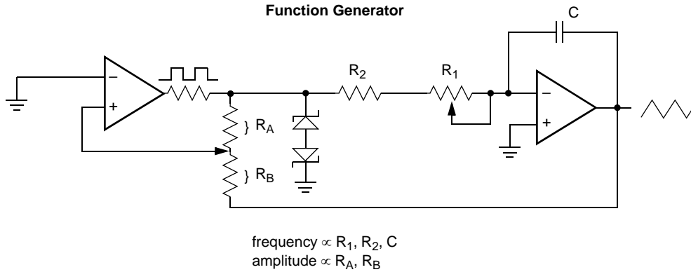
Function Generator
