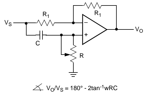
Phase Shifter
