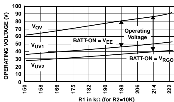
FIGURE 25. OPERATING VOLTAGE vs RESISTOR RATIO
