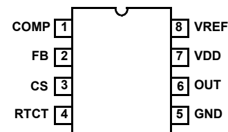
ISL8843 (8 LD SOIC, MSOP) TOP VIEW
