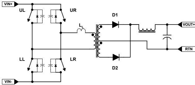
FIGURE 10. IDEALIZED FULL-BRIDGE
