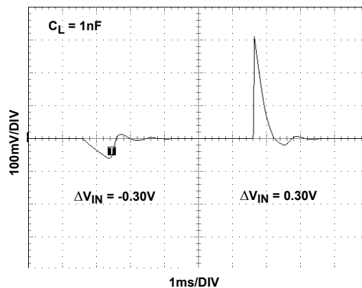
FIGURE 77. LINE TRANSIENT RESPONSE
