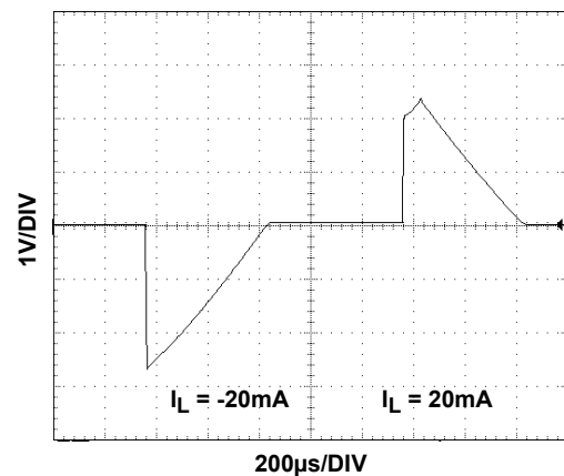
FIGURE 98. LOAD TRANSIENT RESPONSE
