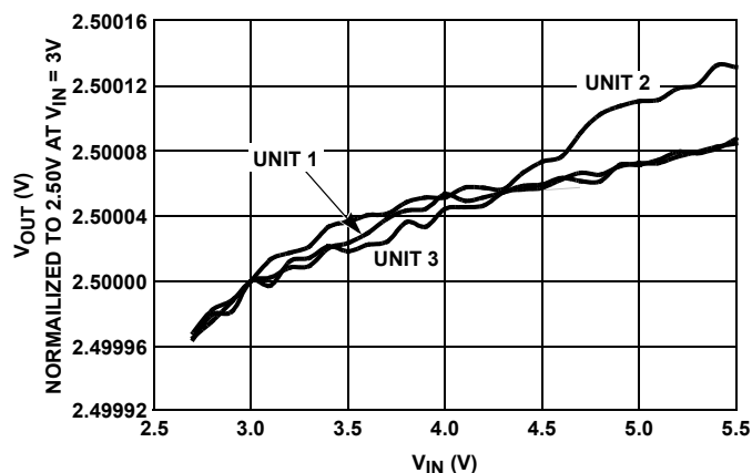
FIGURE 74. LINE REGULATION (3 REPRESENTATIVE UNITS)
