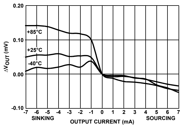
FIGURE 79. LOAD REGULATION
