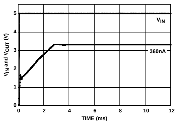
FIGURE 99. TURN-ON TIME (25°C)
