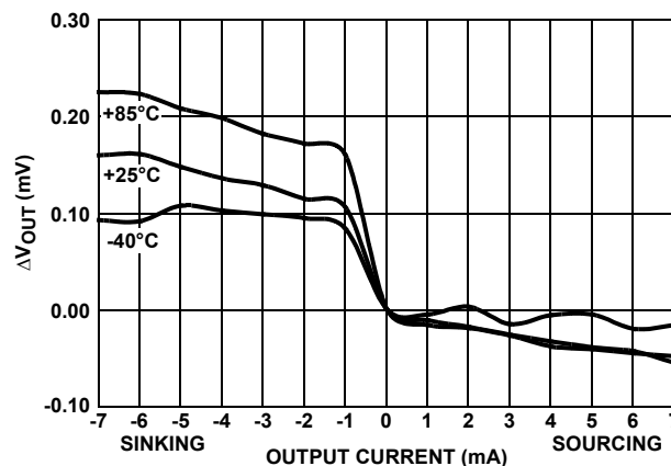
FIGURE 37. LOAD REGULATION
