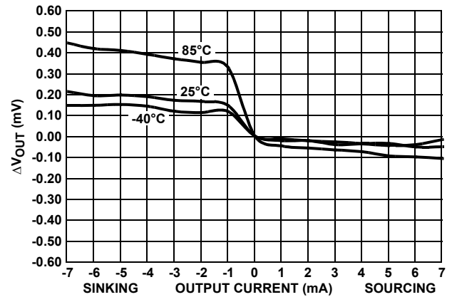
FIGURE 23. LOAD REGULATION
