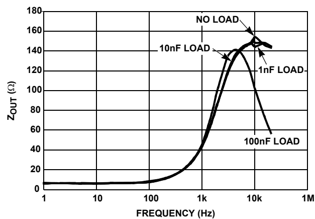
FIGURE 41. Z_{OUT} vs FREQUENCY
