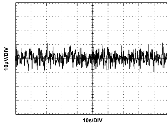
FIGURE 84. V_{OUT} NOISE
