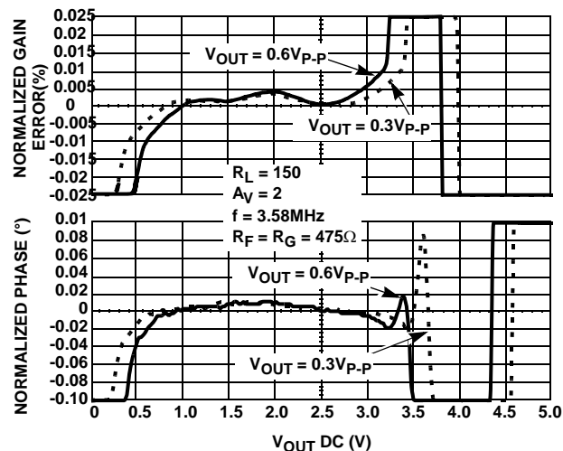
FIGURE 6. DIFFERENTIAL GAIN - PHASE
