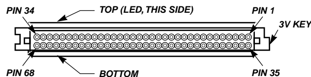
VIEW, LOOKING INTO 68 PIN FEMALE CONNECTOR
