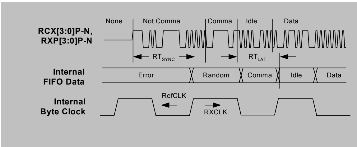
FIGURE 12. BYTE SYNCHRONIZATION
