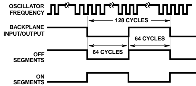
FIGURE 8. DISPLAY WAVEFORMS
