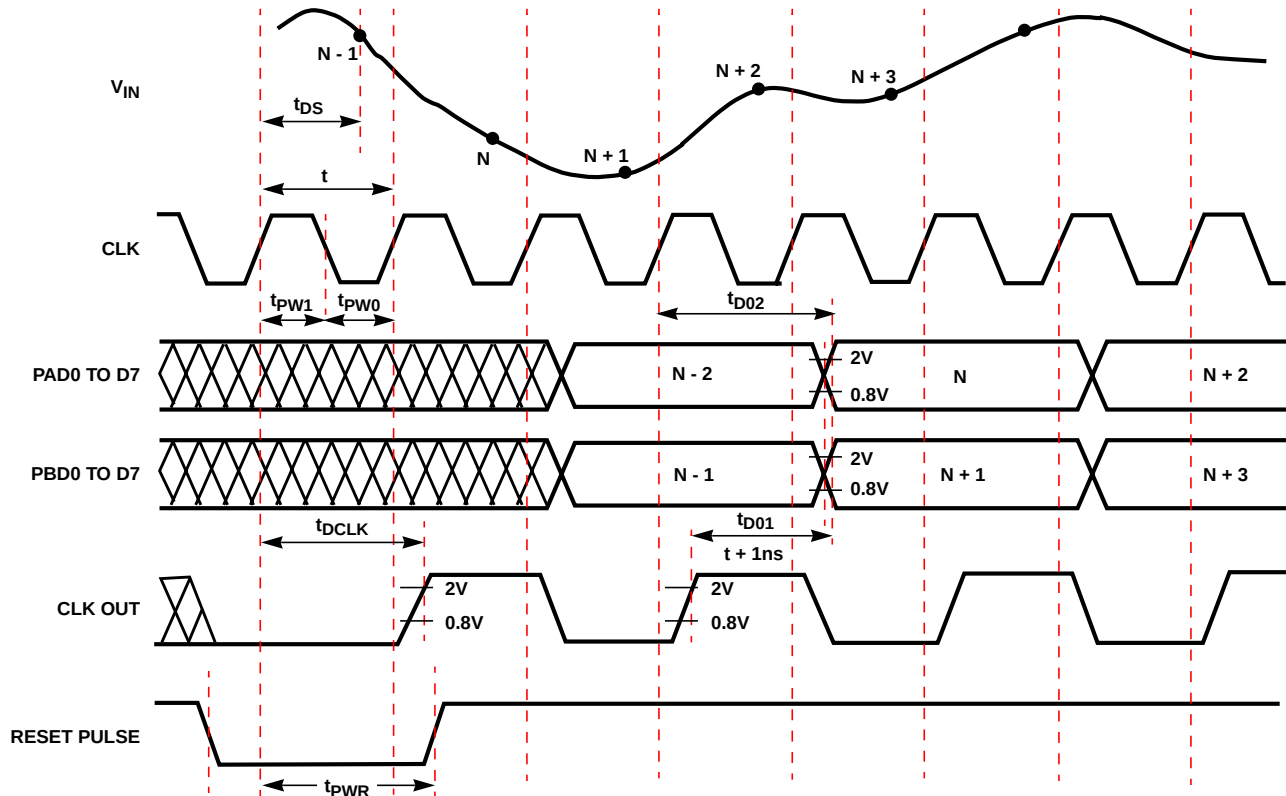
FIGURE 1. DEMUX MODE TIMING CHART ( SELECT1 = V_{CC} )
