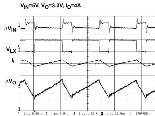
FIGURE 14. SWITCHING WAVEFORMS
