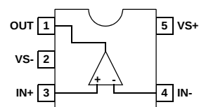
EL5192 (5-PIN SOT-23) TOP VIEW
