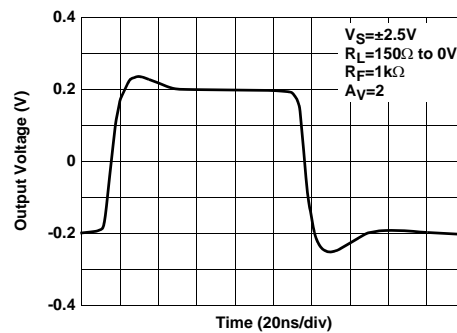
Small Signal Pulse Response (Split Supply)
