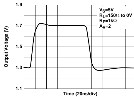
Small Signal Pulse Response (Single Supply)
