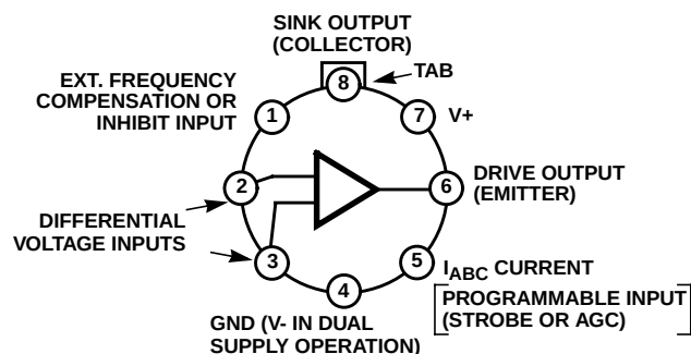
CA3094 (METAL CAN) TOP VIEW
