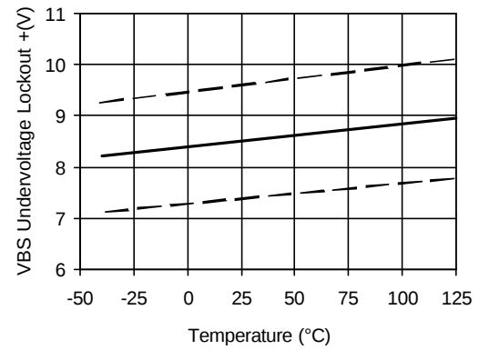
Figure 22. V_{BS} Undervoltage Lockout (+) vs. Temperature
