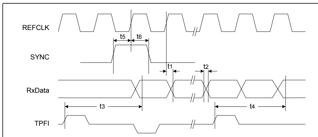
Figure 43. Intel® LXT9785/LXT9785E SMII - 10BASE-T Receive Timing
