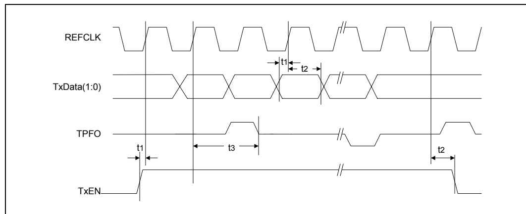
Figure 56. Intel® LXT9785/LXT9785E RMII - 10BASE-T Transmit Timing
