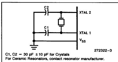
Figure 3. Oscillator Connections
