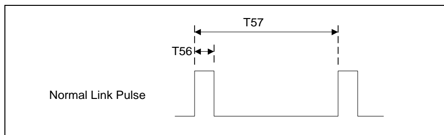
Figure 25. 10BASE-T Normal Link Pulse (NLP) Timings
