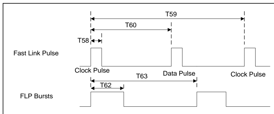
Figure 26. Auto-Negotiation Fast Link Pulse (FLP) Timings
