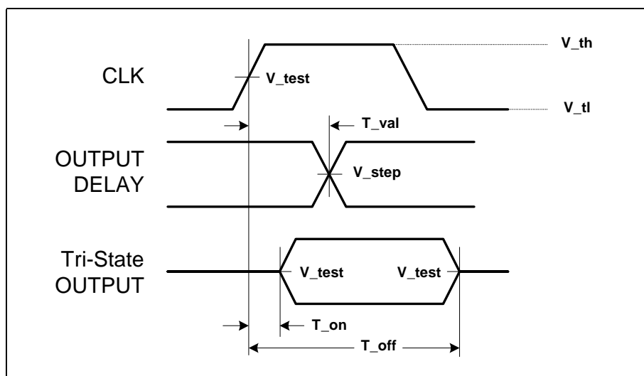
Figure 20. Output Timing Measurement Conditions
