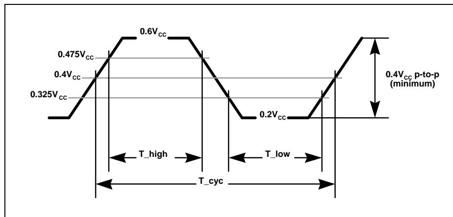
Figure 19. PCI Clock Waveform
