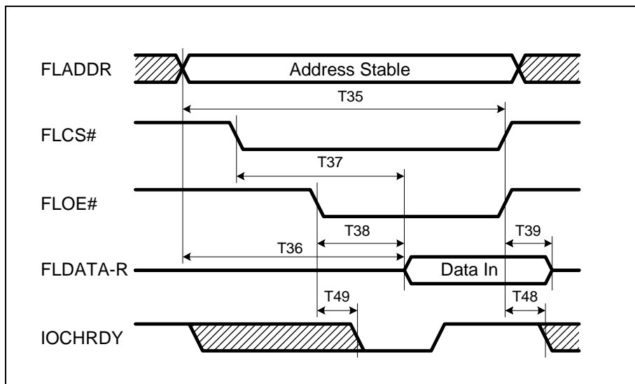
Figure 22. Flash Timings for a Read Cycle
