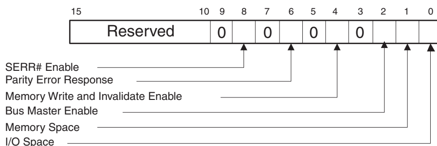
Figure 13. PCI Command Register
