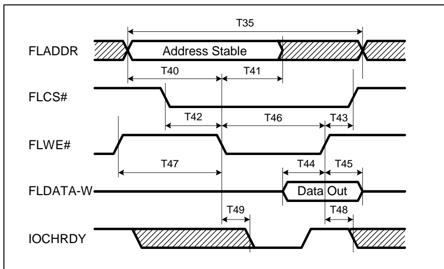
Figure 23. Flash Timings for a Write Cycle
