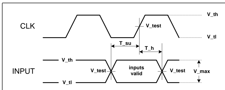
Figure 21. Input Timing Measurement Conditions
