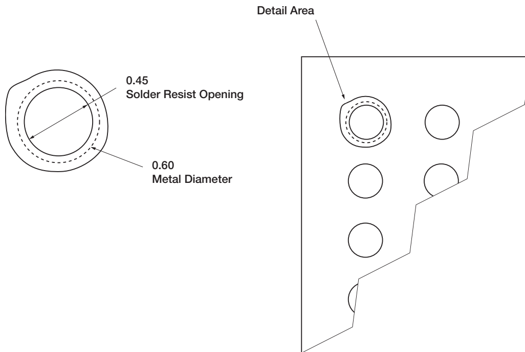
Figure 28. 196 PBGA Package Pad Detail
