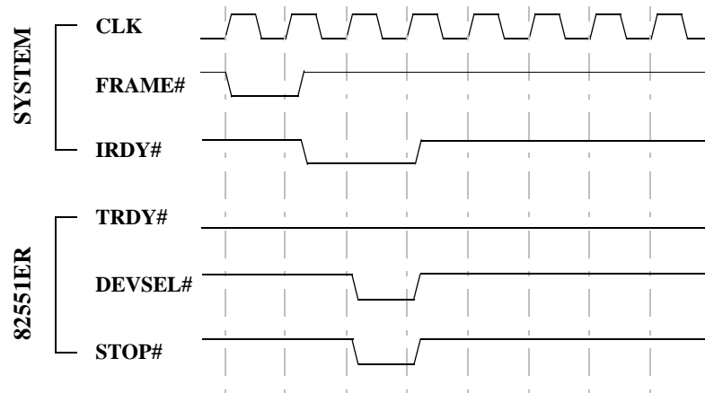
Figure 5. PCI Retry Cycle
