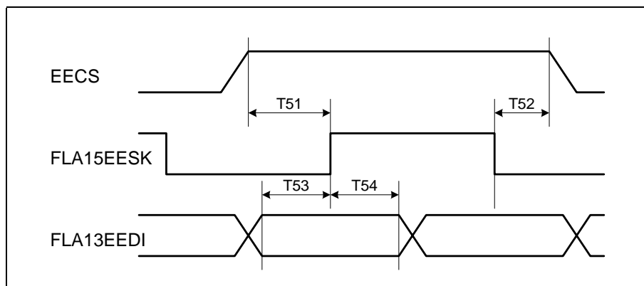
Figure 24. EEPROM Timings
