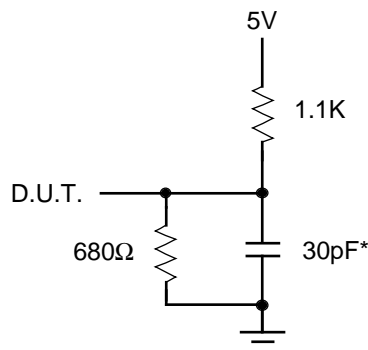
Figure 1. Output Load
