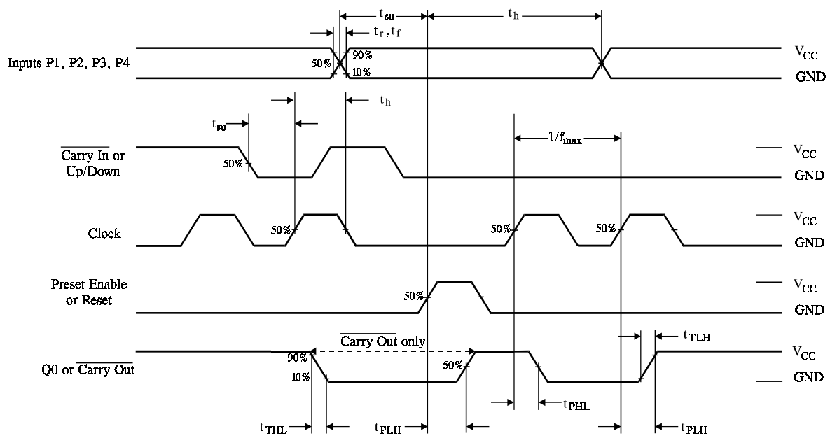
Figure 1. Switching Waveforms
