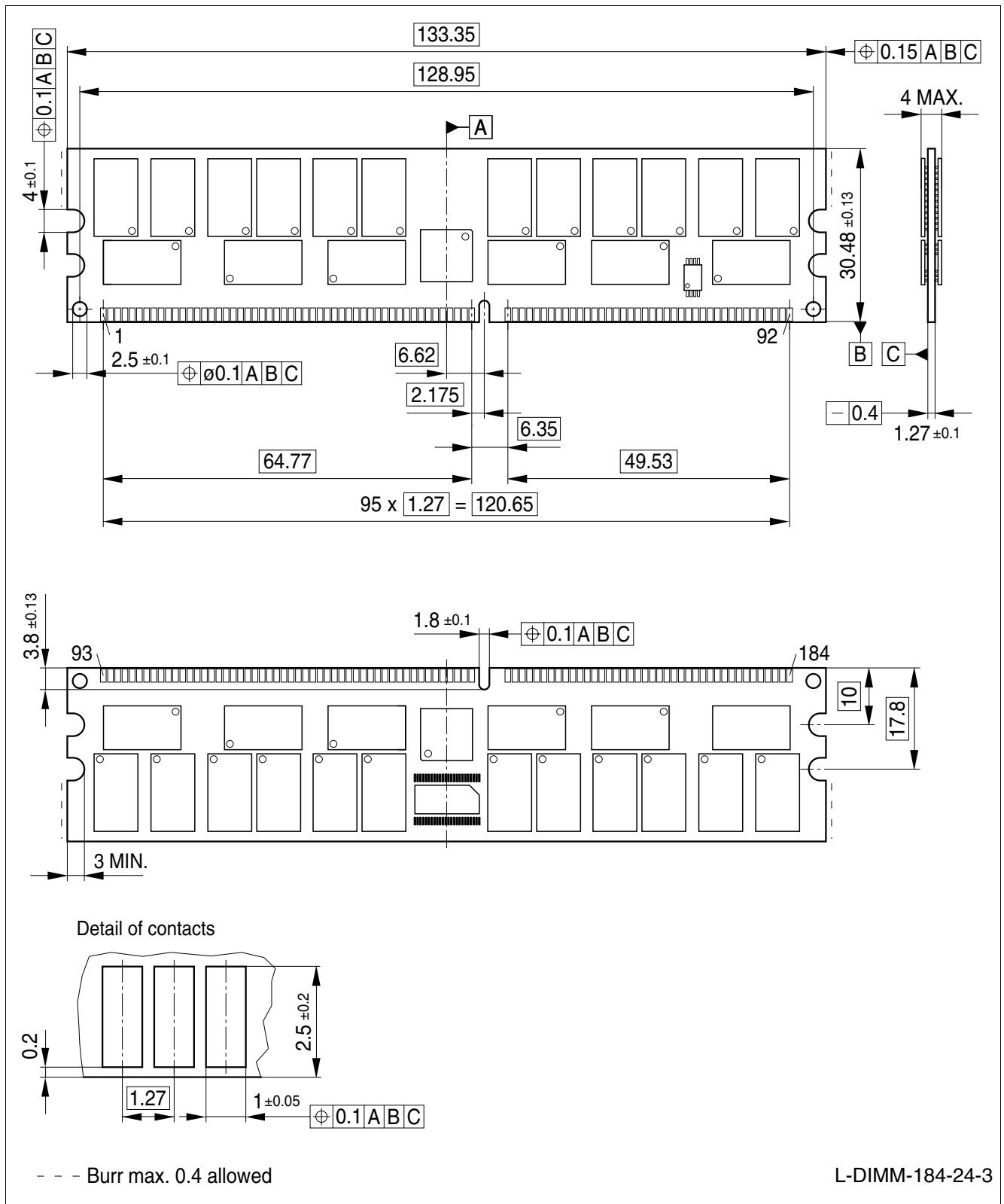
Figure 9 Package Outlines – Raw Card D HYS72D128320GBR–[5/6]–C (2 Ranks ×4)
