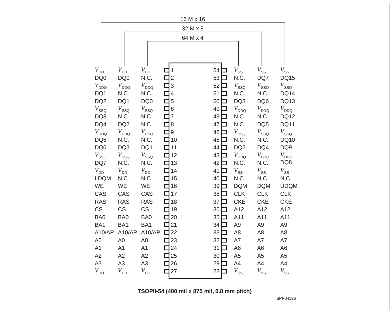
Figure 1 Pinouts P-TSOPII-54
