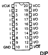
DIP
