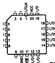
PLCC
