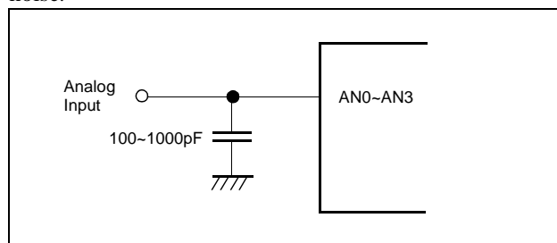
Figure 14-3 Analog Input Pin Connecting Capacitor
