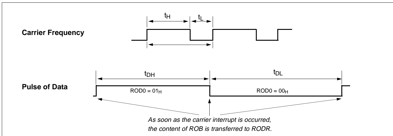
Figure 20-3 Carrier Frequency &amp; Pulse of Data
