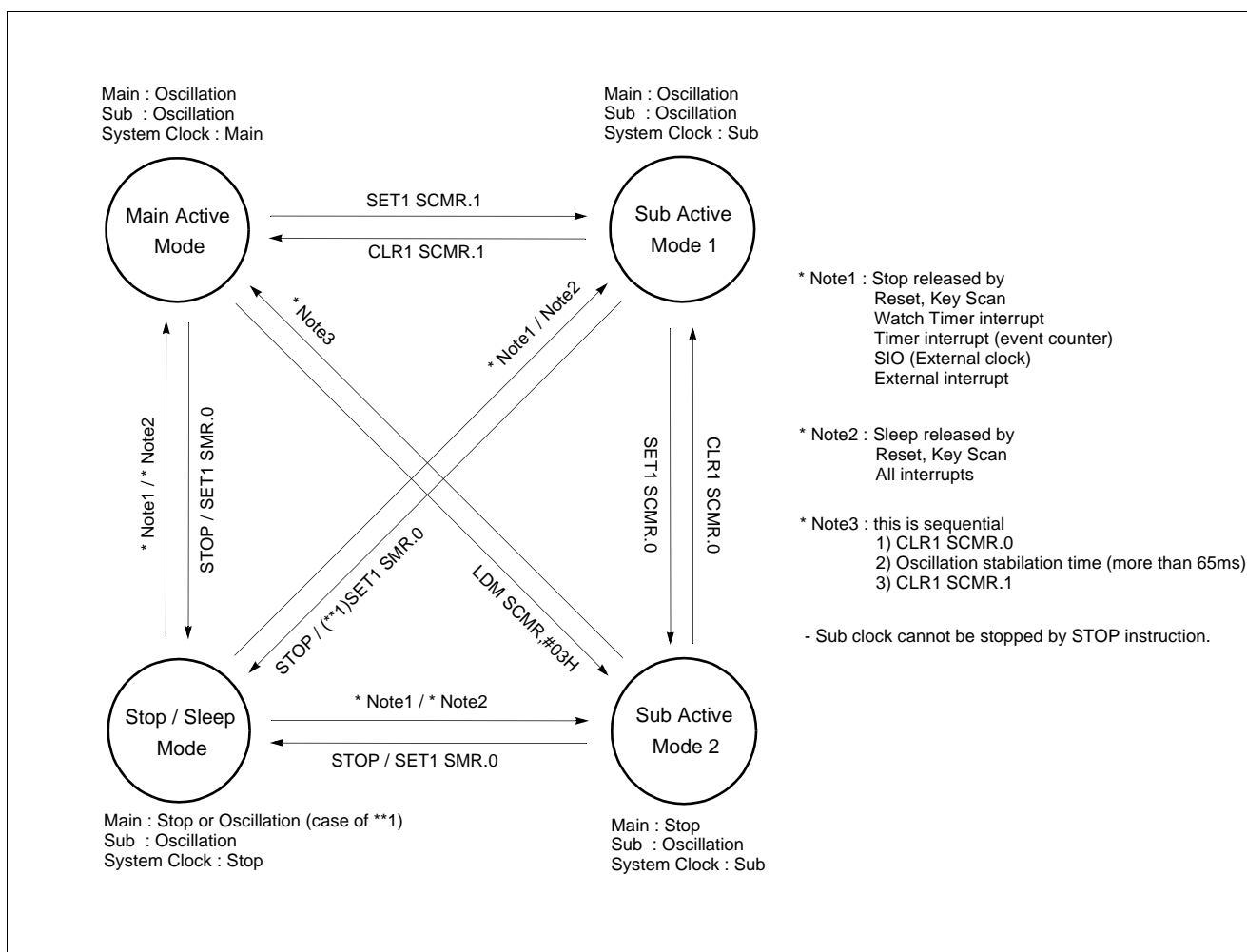
Figure 10-3 Operating Mode
