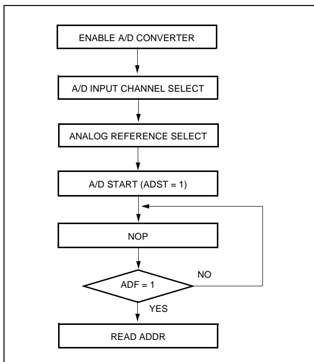
Figure 14-2 A/D Converter Operation Flow
