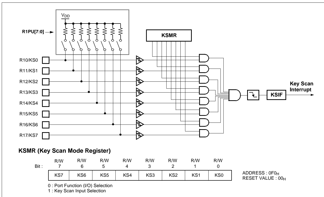
Figure 18-1 Key Scan Interrupt Block Diagram
