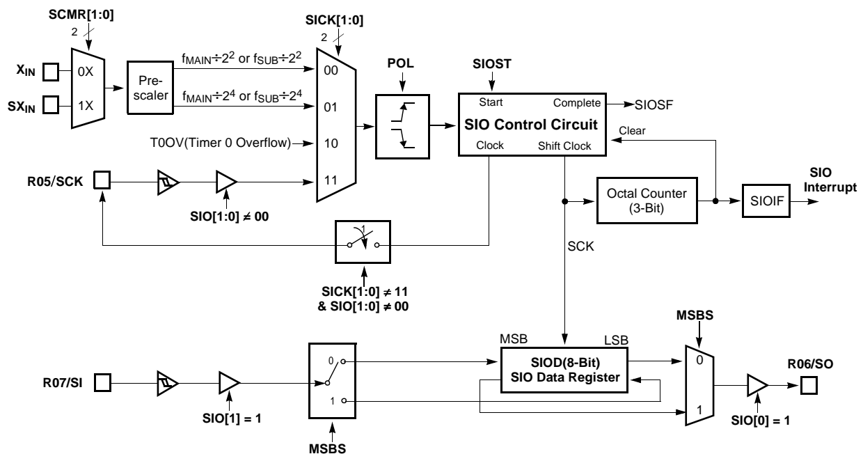
Figure 16-1 SCI Registers and Block Diagram
