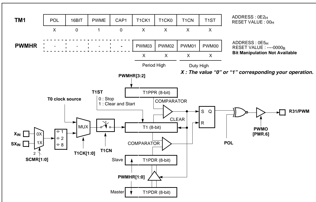
Figure 12-11 PWM Mode
